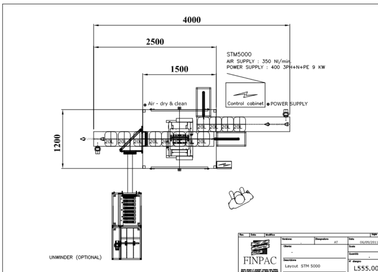
Layout STM 5000
