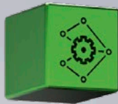
Machine Learning
