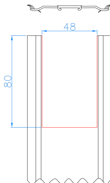
JUNTA INTERIOR HOJA HERMET REF. 1028076
