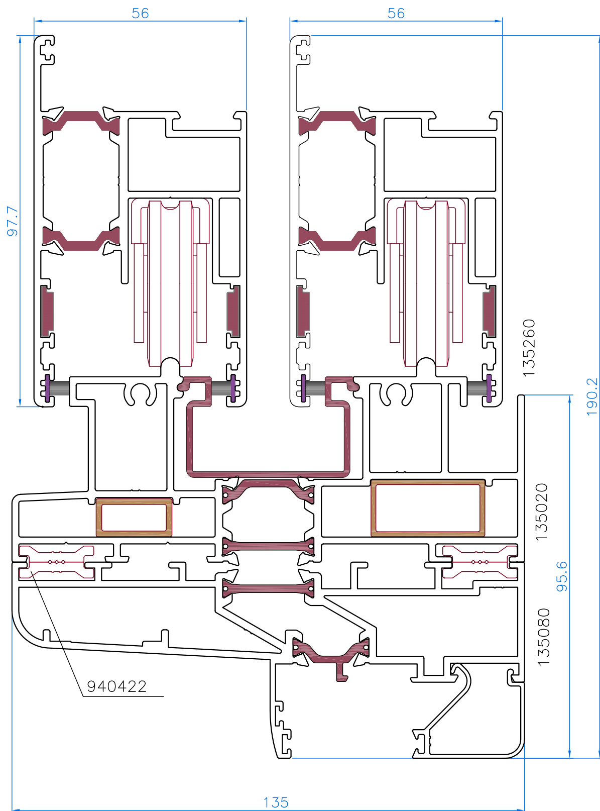
INFERIOR FRAME JOINT WITH FIXED UNION MARCO INFERIOR CON FIJO
