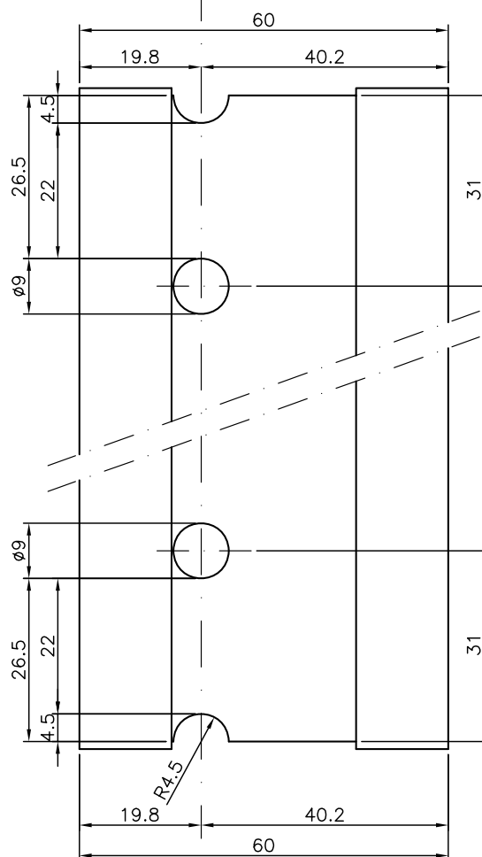
ESCUADRA (ref. 94.92.06)
