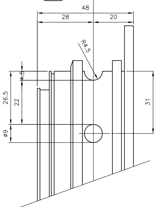
ESCUADRA (ref. 94.92.02)
