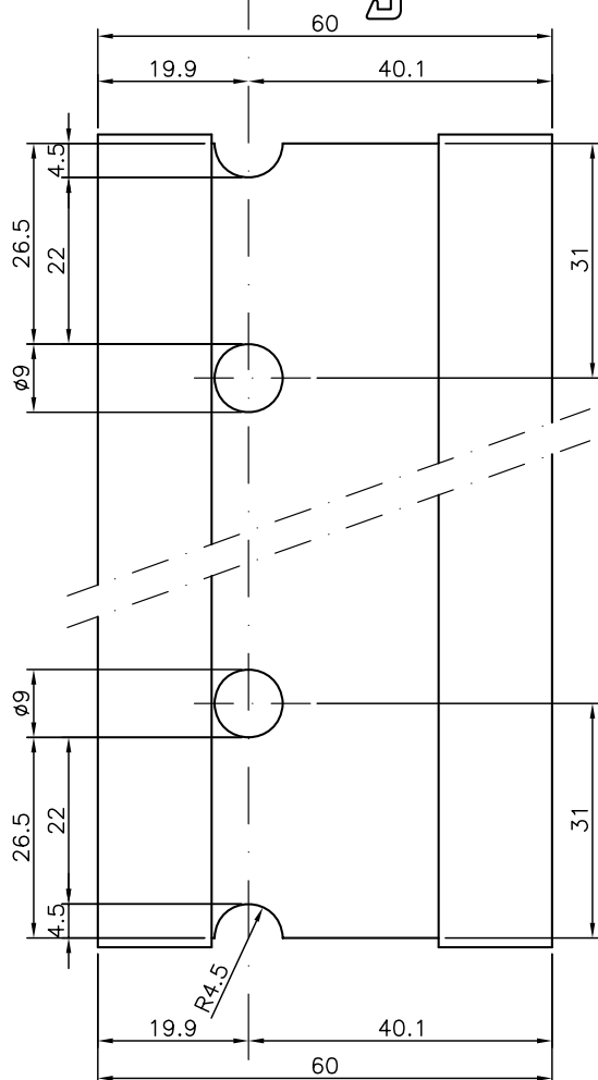
ESCUADRA (ref. 94.92.06)
