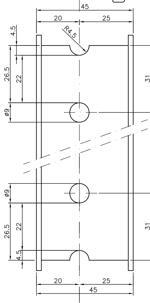
ESCUADRA (ref. 94.92.06)
