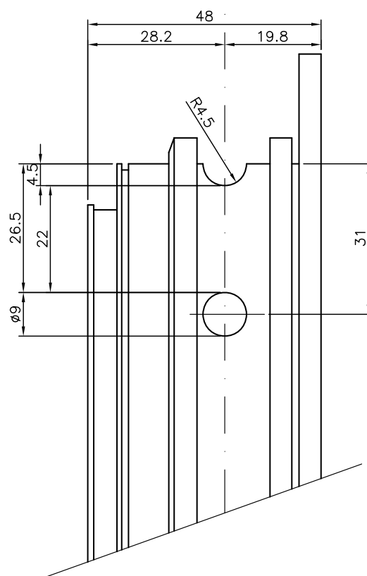
ESCUADRA (ref. 94.92.06)
