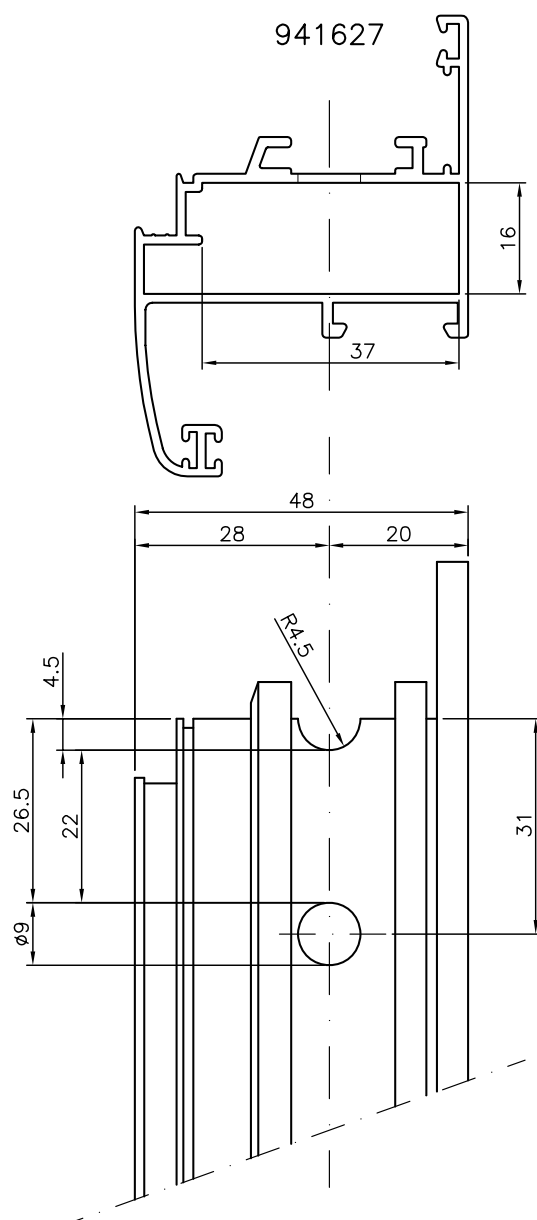
ESCUDRA (ref. 94.92.06)
