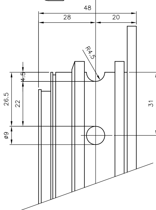
ESCUADRA (ref. 94.92.03)
