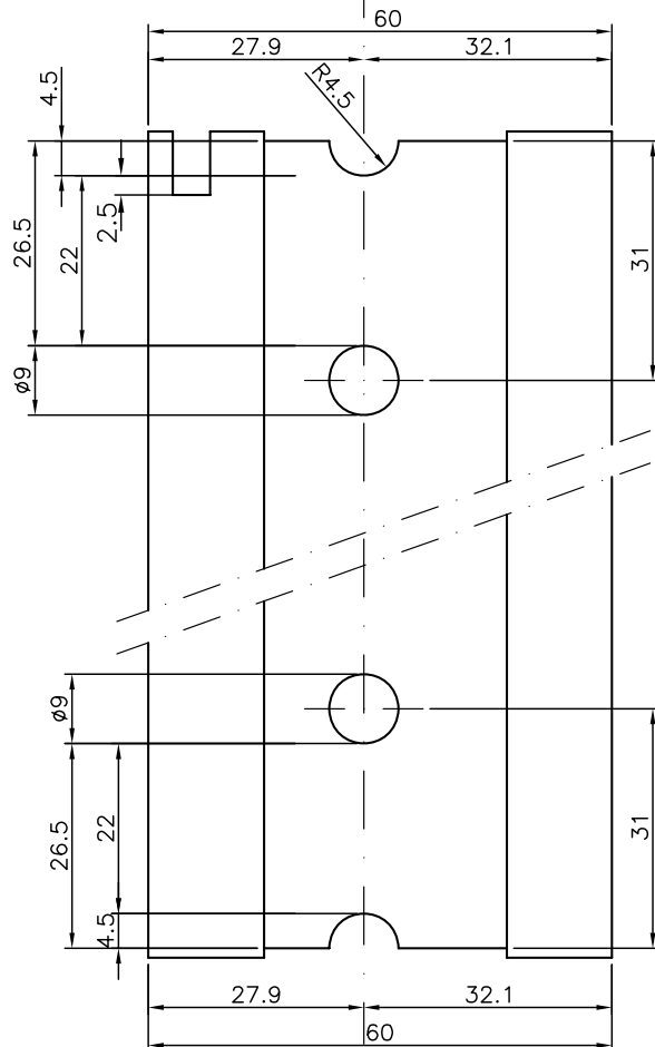
ESCUADRA (ref. 94.92.06)
