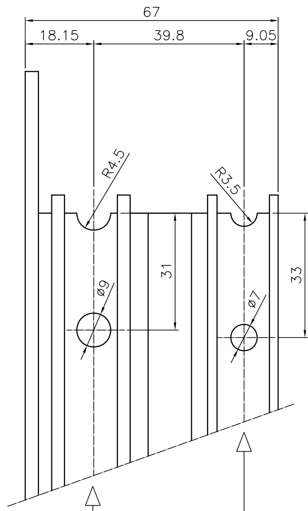
ESCUADRA (ref. 067.041.1)
