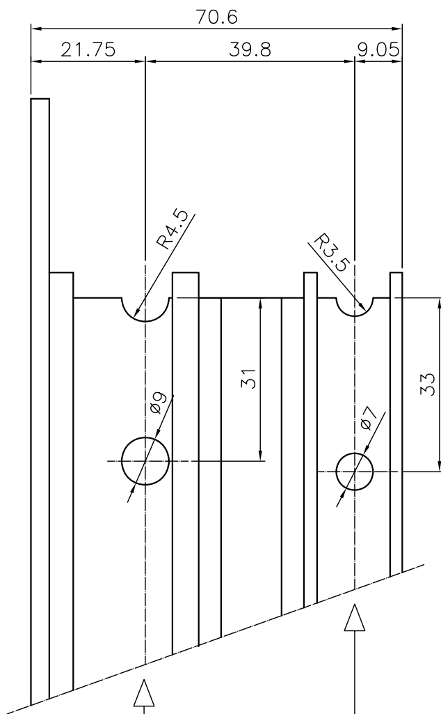
ESCUADRA (ref. 067.041.1)
