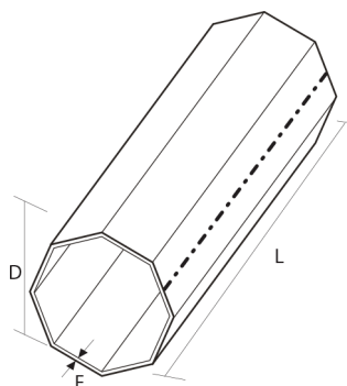
Tubo octogonal (Taladro nacional y export).
