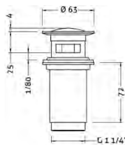
Ref.: 100209 45 Válvula click 1 1/4" con/sin rebosadero 1 1/4" click valve with/out overflow
