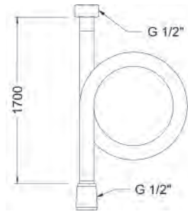
Ref.: 100140 30 Flexo H 1/2" - H 1/2" 1,70 m. PVC antirrotura F 1/2" - F 1/2" PVC flexible hose 1.70 m anti- breaking
