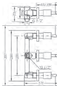
Ref.: 68116 12 45 66 Grupo ducha empotrado 8\"/> Built-in 8\" shower mixer with diverter Box: 1
