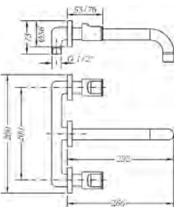
Ref.: 68132 07 45 66 Grupo de lavabo empotrado caño 22 cm Built-in wash-basin with 22 cm pipe spout
