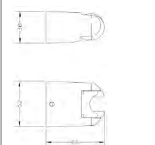
Ref.: 100068 45 Soporte ducha ovalado Oval shower holder
