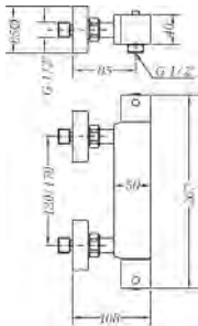
Ref.: 67110 26 45 67 Termostática ducha sin kit Thermostatic shower mixer without kit
