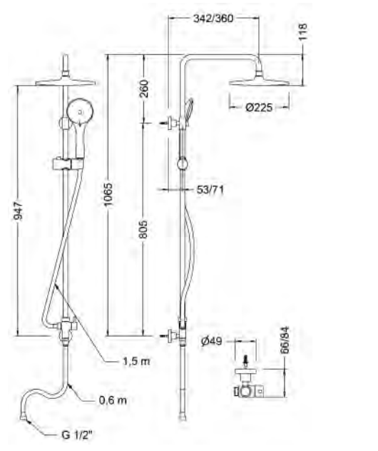
Ref.: 1744 45 Set columna fija con kit Fixed column set with kit
