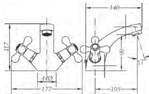
Ref.: 68505 09 45 66 Monobloc de lavabo Wash-basin mixer
