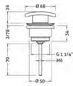
Ref.: 100204 45 Válvula click Kenjo 1 1/4" 1 1/4" Kenjo click valve
