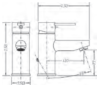
Ref.: 65135 29 45 66 Monomando de lavabo Single lever wash-basin mixer
