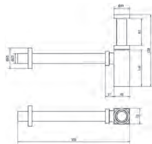
Ref.: 1621 07 Sifon botella para lavabo y bidé 1 1/4" 1 1/4" bidet and wash-basin siphon
