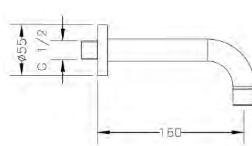
Ref.: 68911 45 Caño mural tubo recto 16 cm Wall mounted pipe spout 16 cm
