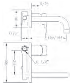
Ref.: 64131 16 45 66 Monomando de lavabo empotrado caño 16 cm Built-in wash-basin mixer 16 cm spout
