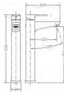
Ref.: 63136 26 45 66 Monomando de lavabo alto High single lever wash-basin mixer
