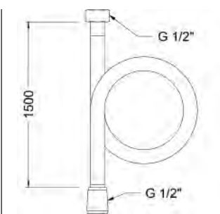
Ref.: 9908 0206 Flexo H 1/2" - H 1/2" 1,5 m cromado F 1/2" - F 1/2" 1.5 m chromed flexible hose
