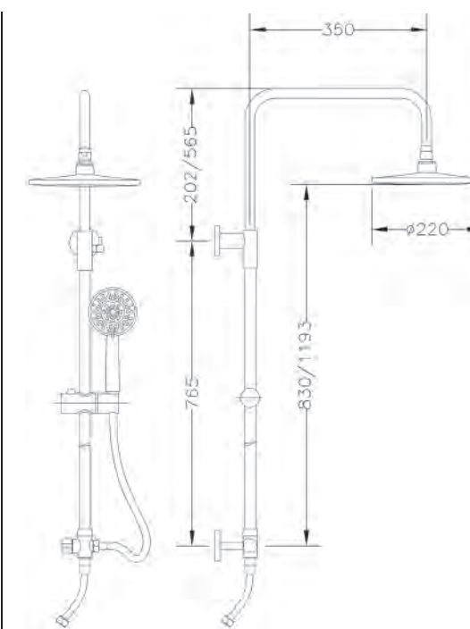
Ref.: 1745 45 Set columna extensible con ducha, soporte y flexo Extensible column set with shower, holder and flexible hose
