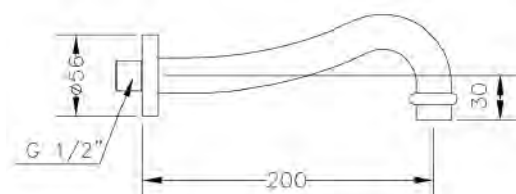
Ref.: 68914 45 Caño mural tubo retro 20 cm Wall mounted retro pipe spout 20 cm
