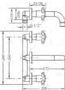
Ref.: 68131 08 45 66 Grupo de lavabo empotrado caño 16 cm Built-in wash-basin mixer with 16 cm pipe spout
