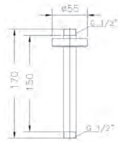
Ref.: 1671 45 Brazo a techo redondo 15 cm Round roof arm 15 cm Box: 1 | Carton: 20 | Pallet: 600
