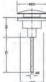
Ref.: 100202 45 Tapa universal "Click remove" "Click remove" universal cover
