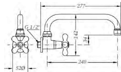
Ref.: 68580 09 45 66 Grifo mural fregadera caño tubo alto 24 cm Wall sink tap with tube spout 24 cm
