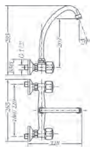
Ref.: 68103 11 45 66 Grupo mural fregadera 20 cm caño tubo alto vertical 20 cm wall sink mixer with swan neck spout Box: 1 | Carton: 10 | Pallet: 240
