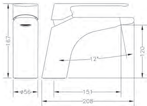
Ref.: 62130 08 45 66 Monomando de lavabo Single lever wash-basin mixer
