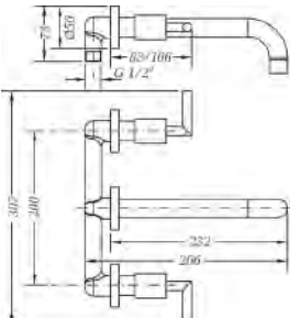
Ref.: 68132 12 45 66 Grupo de lavabo empotrado caño 22 cm Built-in wash-basin mixer with 22 cm pipe spout Box: 1
