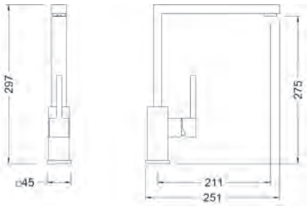
Ref.: FRK63400 Monomando de fregadera cartucho 25 Single lever sink mixer 25 cartridge
