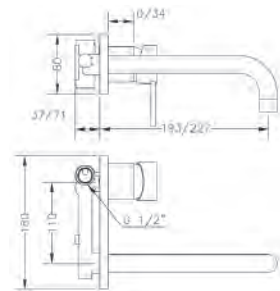
Ref.: 65132 29 45 66 Monomando de lavabo empotrado caño 22 cm Built-in wash-basin mixer 22 cm spout
