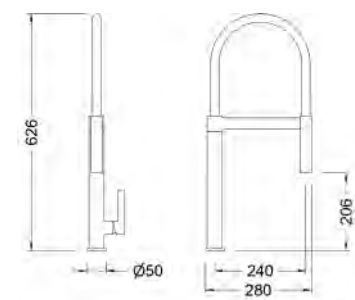
Ref.: 65219 40 60 66 Monomando de fregadera cartucho 25 Single lever sink mixer 25 cartridge
