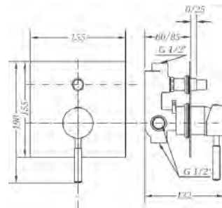
Ref.: 65116 18 45 66 Monomando de baño empotrado con inversor Built-in single lever mixer bath with diverter
