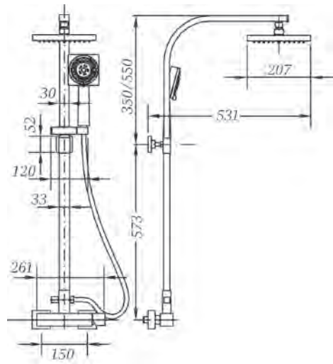
Ref.: CM63110 26 Columna monomando extensible con kit Single lever extensible column with kit
