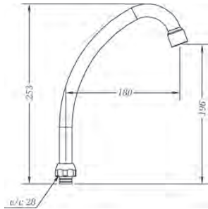
Ref.: 68903 45 Caño tubo vertical Swan neck spout
