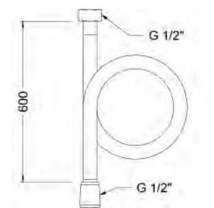
Ref.: 9908 0203 Flexo H1/2" - H1/2" 60cm F1/2"-F1/2" 60cm Flexible hose
