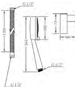
Ref.: 100698 45 Kit de ducha Kenjo, flexo, soporte y ducha 3 jets Kenjo shower set, flexible hose, holder and 3 jets handshower
