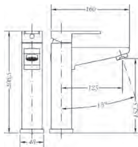
Ref.: 63134 26 45 66 Monomando de lavabo medio alto Medium height single lever wash-basin mixer
