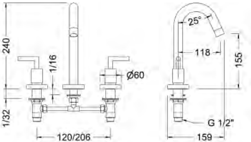
Ref.: 68125 12 45 66 Batería de lavabo caño inclinado Widespread wash-basin mixer with sloping pipe spout Box: 1
