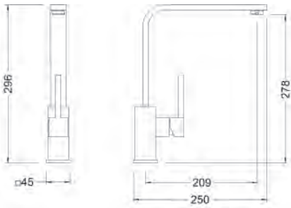
Ref.: FRK63401 Monomando de fregadera cartucho 25 Single lever sink mixer 25 cartridge
