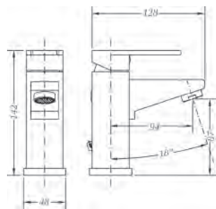
Ref.: 63130 26 45 66 Monomando de lavabo Single lever wash-basin mixer
