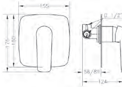
Ref.: 62115 31 45 66 Monomando de ducha empotrado Built-in single lever shower mixer
