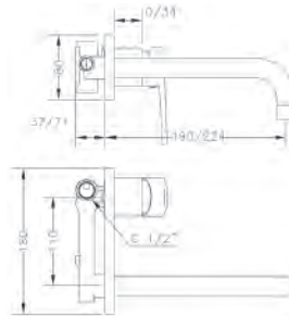
Ref.: 64132 16 45 66 Monomando de lavabo empotrado caño 22 cm Built-in wash-basin mixer 22 cm spout
