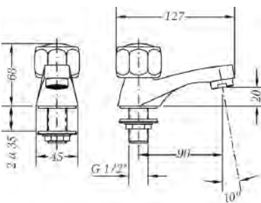
Ref.: 68180 11 45 66 Grifo de lavabo Wash-basin tap
