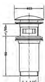
Ref.: 100210 45 Válvula click 1 1/4" con/sin rebosadero 1 1/4" click valve with/out overflow
