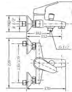
Ref.: 60100 22 45 66 Monomando de baño con kit Single lever bath mixer with kit
