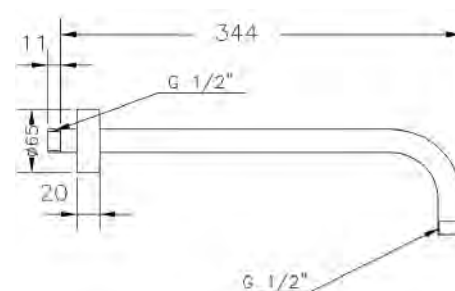
Ref.: B65114 18 Brazo pared redondo 24 cm Round arm 24 cm
