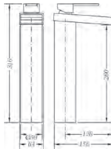
Ref.: 63138 26 45 66 Monomando de lavabo cascada alto High waterfall single lever wash-basin mixer
