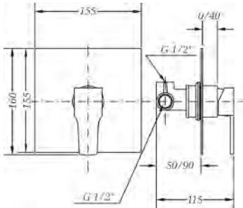
Ref.: 63115 26 45 66 Monomando de ducha empotrado Built-in single lever shower mixer
