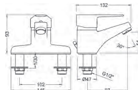
Ref.: 60188 28 45 66 Monomando de lavabo centerset 4" Single lever wash-basin mixer 4" centerset
