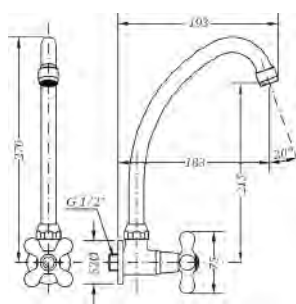
Ref.: 68575 09 45 66 Grifo fregadera mural caño tubo vertical Wall sink tap with swan neck spout
