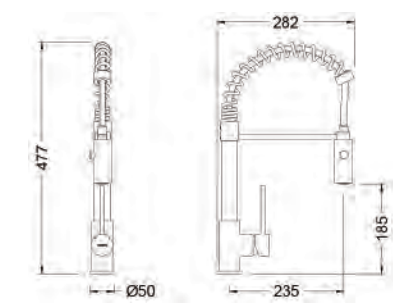
Ref.: 65211 18 45 66 Monomando de fregadera con muelle Single lever sink mixer with spring
