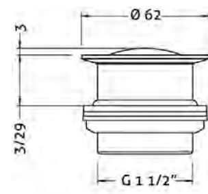
Ref.: 100208 45 Válvula click 1 1/4" bañera 1 1/4" bath click valve
