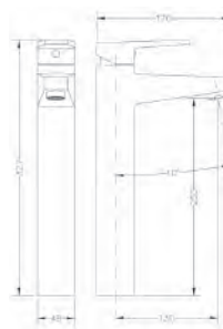
Ref.: 64136 16 45 66 Monomando de lavabo alto High single lever wash-basin mixer
