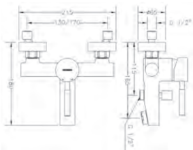
Ref.: 65100 18 45 66 Monomando de baño con kit Single lever bath mixer with kit
