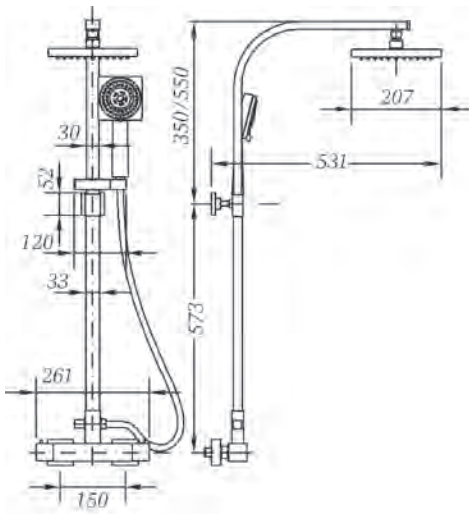
Ref.: CT67110 26 Columna termostática extensible con kit Thermostatic extensible column with kit
