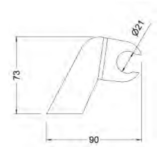
Ref.: 100152 45 00 Soporte ducha Combi Combi shower holder
