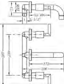
Ref.: 68131 12 45 66 Grupo de lavabo empotrado caño 16 cm Built-in wash-basin mixer with 16 cm pipe spout Box: 1
