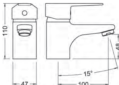
Ref.: 60130 28 45 66 Monomando de lavabo Single lever wash-basin mixer
