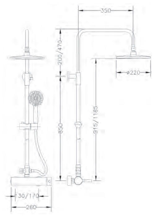
Ref.: CM65110 18 Columna monomando extensible con kit Single lever extensible column with kit
