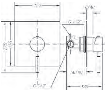
Ref.: 65115 18 45 66 Monomando de ducha empotrado Built-in single lever shower mixer
