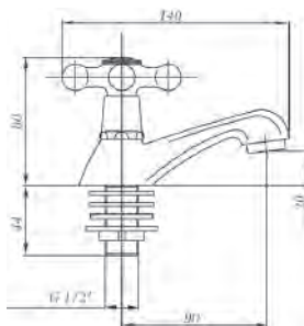
Ref.: 68500 09 45 66 Grifo lavabo Wash-basin tap
