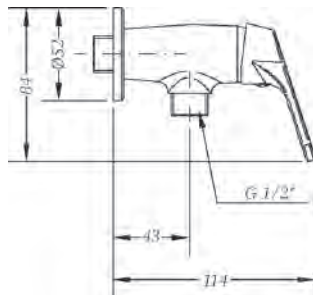
Ref.: 60001 22 45 67 Grifo bide mural 1 agua 1 water wall bidet
