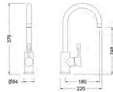
Ref.: 65203 18 60 66 Monomando de fregadera inox caño cisne Stainless steel single lever sink mixer with swan spout Box: 1 | Carton: 5 | Pallet: 60
