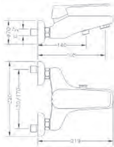
Ref.: 62100 08 45 67 Monomando de baño sin kit Single lever bath mixer without kit
