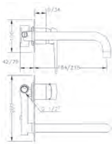
Ref.: 62132 31 45 66 Monomando de lavabo empotrado caño 22 cm Built-in wash-basin mixer 22 cm spout
