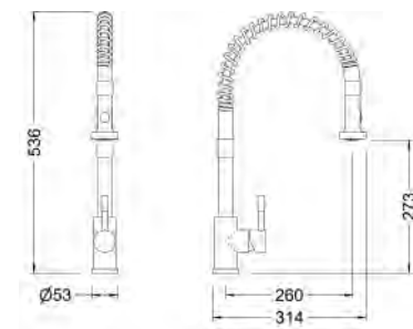
Ref.: 65207 18 60 66 Monomando de fregadera inox con muelle y ducha extraíble Stainless steel single lever sink mixer with spring and pull-out sprayer Box: 1 | Carton: 4
