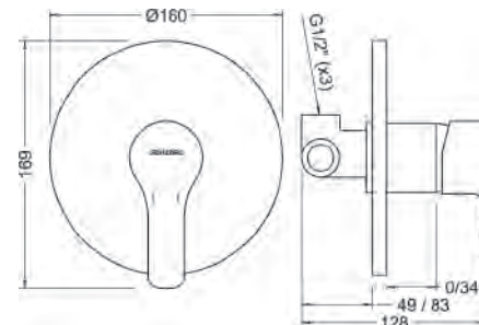
Ref.: 61115 28 45 66 Monomando de ducha empotrado Built-in single lever shower mixer
