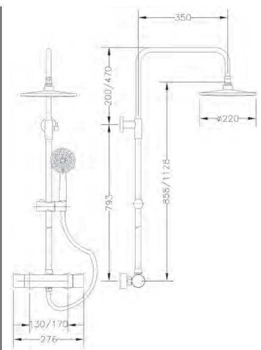
Ref.: CT67110 18 Columna termostática extensible con kit Thermostatic extensible column with kit
