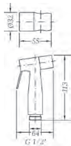
Ref.: 100694 45 Kit ducha sanitaria Sanitary shower kit Box: 1 | Carton: 22 | Pallet: 268
