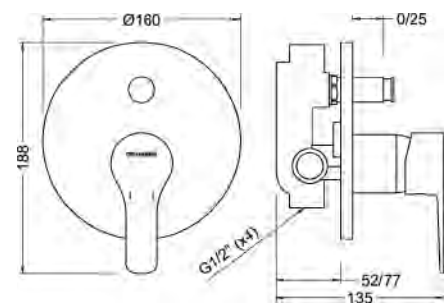
Ref.: 61116 28 45 66 Monomando de baño empotrado con inversor Built-in single lever bath mixer with diverter
