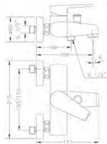
Ref.: 64100 16 45 66 Monomando de baño con kit Single lever bath mixer with kit
