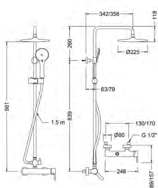
Ref.: CM65110 19 Columna monomando fija con kit Single lever fixed column with kit
