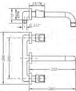
Ref.: 68132 08 45 66 Grupo de lavabo empotrado caño 22 cm Built-in wash-basin mixer with 22cm pipe spout
