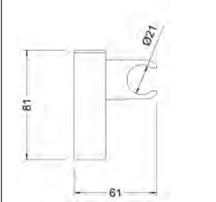
Ref.: 100149 45 Soporte ducha Kenjo Kenjo shower holder
