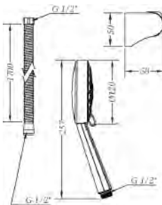
Ref.: 100699 45 Kit de ducha Tau, flexo, soporte y ducha 5 jets Tau shower set, flexible hose, holder and 5 jets handshower
