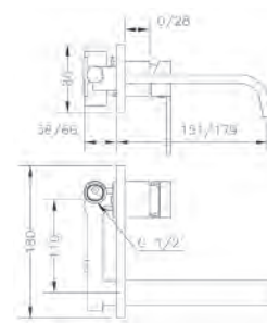
Ref.: 63131 26 45 66 Monomando de lavabo empotrado caño 16 cm Built-in wash-basin mixer 16 cm spout
