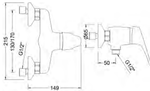
Ref.: 60110 22 45 66 Monomando de ducha con kit Single lever shower mixer with kit
