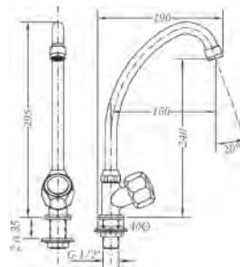
Ref.: 68003 11 45 66 Grifo fregadera encimera caño tubo vertical Deck sink tap with swan neck spout Box: 1 | Carton: 10 | Pallet: 240
