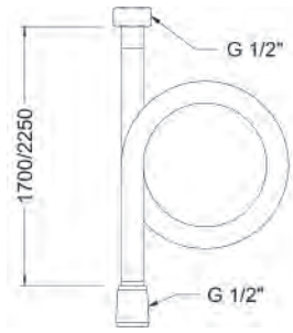
Ref.: 100137 60 00 Flexo extensible H 1/2" - H 1/2" 1,70 - 2,25 m inoxidable F 1/2" - F 1/2" Extensible stainless steel flexible hose 1.70 to 2.25 m
