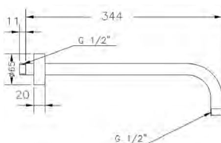
Ref.: B65113 18 Brazo pared redondo 35 cm Round wall arm 35 cm
