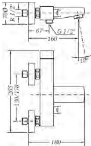
Ref.: 63100 26 45 67 Monomando de baño sin kit Single lever bath mixer without kit
