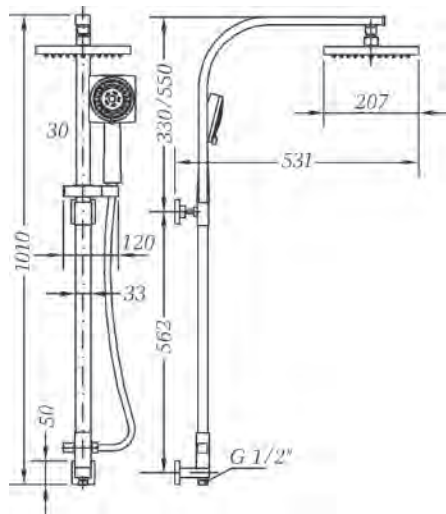
Ref.: 1746 45 Set columna extensible con ducha, soporte y flexo Extensible column set with shower, holder and flexible hose
