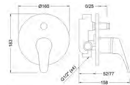
Ref.: 61116 22 45 66 Monomando de baño empotrado con inversor Built-in single lever bath mixer with diverter
