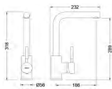
Ref.: 65214 18 45 66 Monomando de fregadera cartucho 40 Single lever sink mixer 40 cartridge
