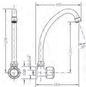
Ref.: 68083 11 45 66 Grifo fregadera mural caño tubo vertical Wall sink tap with swan neck spout Box: 1 | Carton: 10 | Pallet: 240
