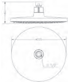
Ref.: R65112 18 Rociador redondo 22 cm Round shower head 22 cm Box: 1 | Carton: 24 | Pallet: 144
