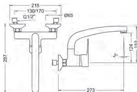
Ref.: 61192 28 45 66 Monomando de fregadera mural 15 cm Wall single-lever sink mixer 15 cm
