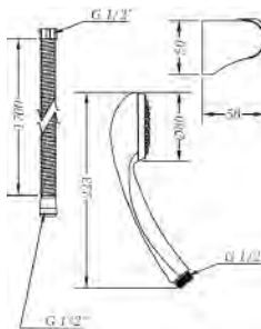
Ref.: 100697 45 Kit de ducha GE2, flexo, soporte y ducha 1 jet GE2 shower set, flexible hose, holder and 1 jet handshower
