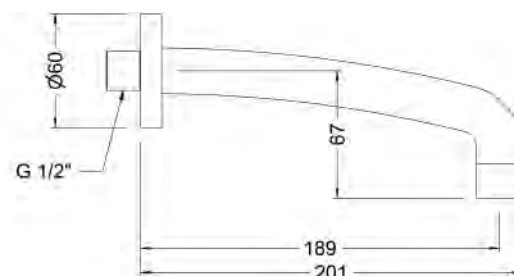
Ref.: 68913 45 Caño mural tubo inclinado 20 cm Wall mounted sloping pipe spout 20 cm
