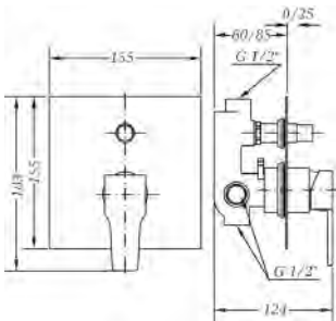
Ref.: 63116 26 45 66 Monomando de baño empotrado con inversor Built-in single lever bath with mixer with diverter
