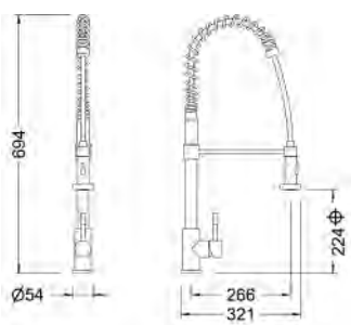
Ref.: 65211 18 60 66 Monomando de fregadera inox con muelle Stainless steel single lever sink mixer with spring
