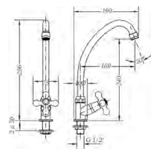
Ref.: 68585 09 45 66 Grifo fregadera encimera caño tubo vertical Deck sink tap with swan neck spout
