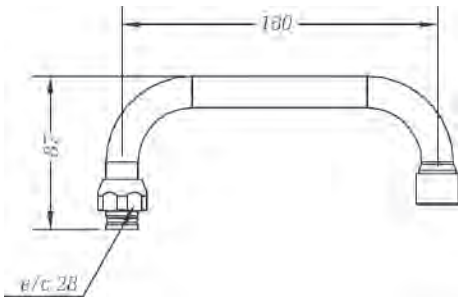
Ref.: 68901 45 Caño alto tubo 18 cm High tube spout 18 cm
