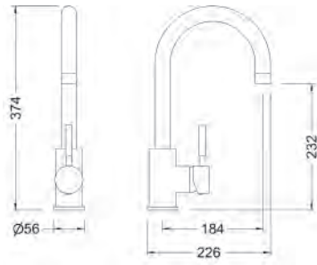
Ref.: 65203 18 45 66 Monomando de fregadera cartucho 40 Single lever sink mixer 40 cartridge Box: 1 | Carton: 5 | Pallet: 90
