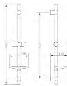
Ref.: 1636 45 Barra ducha TAU TAU shower bar
