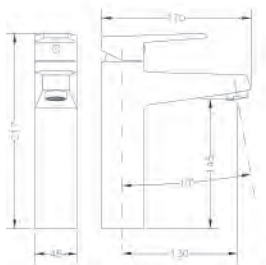
Ref.: 64134 16 45 66 Monomando de lavabo medio alto Medium height single lever wash-basin mixer
