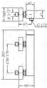
Ref.: 63110 26 45 67 Monomando de ducha sin kit Single lever shower mixer without kit
