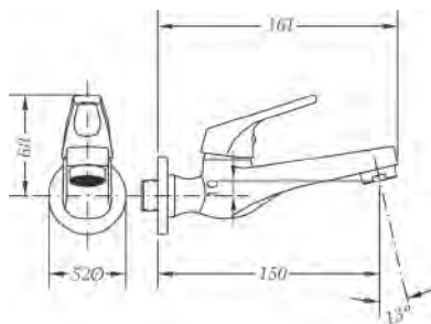
Ref.: 1003 04 Grifo lavabo mural 1 agua cartucho 25 One-water wall wash-basin tap 25 cartridge
