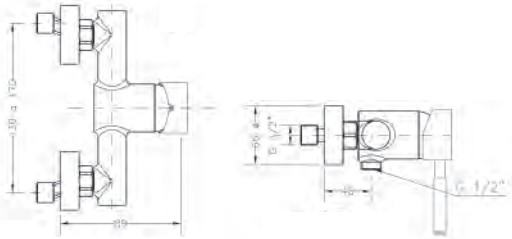
Ref.: 65110 18 45 66 Monomando de ducha con kit Single lever shower mixer with kit
