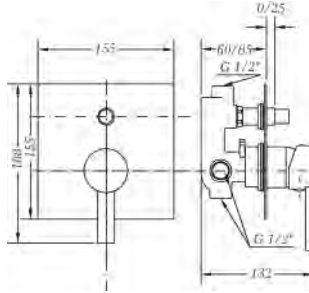
Ref.: 65116 29 45 66 Monomando de baño empotrado con inversor Built-in single lever bath mixer with diverter
