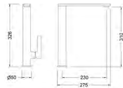
Ref.: 65215 40 60 66 Monomando de fregadera cartucho 25 Single lever sink mixer 25 cartridge
