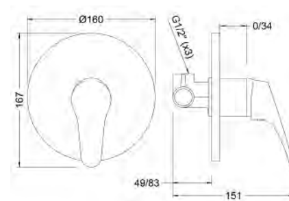
Ref.: 61115 22 45 66 Monomando de ducha empotrado Built-in single lever shower mixer
