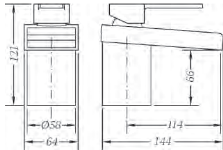
Ref.: 63137 26 45 66 Monomando de lavabo cascada Waterfall single lever wash-basin mixer
