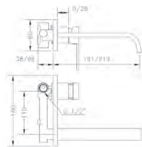
Ref.: 63132 26 45 66 Monomando de lavabo empotrado caño 22 cm Built-in wash-basin mixer 22 cm spout
