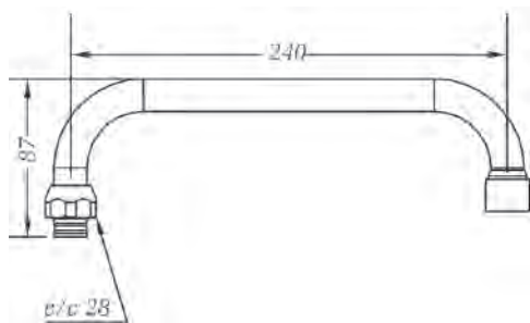
Ref.: 68902 45 Caño alto tubo 24 cm High tube spout 24 cm
