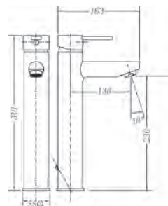
Ref.: 65136 29 45 66 Monomando de lavabo alto High single lever wash-basin mixer
