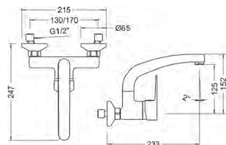
Ref.: 61190 28 45 66 Monomando de fregadera mural 15 cm caño corto Wall single lever sink mixer 15 cm short spout
