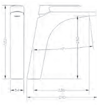
Ref.: 62136 08 45 66 Monomando de lavabo alto High single lever wash-basin mixer
