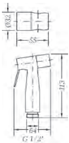
Ref.: 100694 60 Kit ducha sanitaria inox Inox sanitary shower kit Box: 1 | Carton: 22 | Pallet: 268
