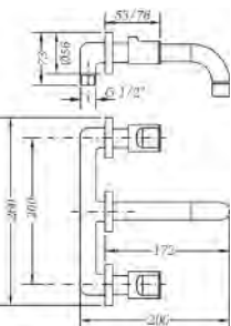
Ref.: 68131 07 45 66 Grupo de lavabo empotrado caño 16 cm Built-in wash-basin mixer with 16 cm pipe spout
