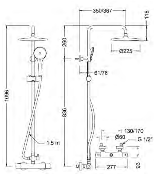
Ref.: CT67110 19 Columna termostática fija con kit Thermostatic fixed column with kit
