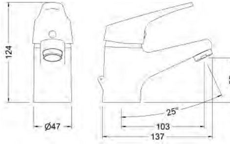
Ref.: 60130 22 45 66 Monomando de lavabo Single lever wash-basin mixer
