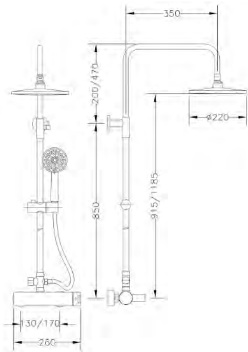
Ref.: CM65110 29 Columna monomando extensible con kit Single lever extensible column with kit
