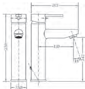
Ref.: 65134 29 45 66 Monomando de lavabo medio alto Medium height single lever wash-basin mixer
