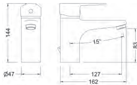
Ref.: 60134 28 45 66 Monomando de lavabo medio alto Medium height single lever wash-basin mixer
