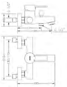
Ref.: 65100 29 45 66 Monomando de baño con kit Single lever bath mixer with kit
