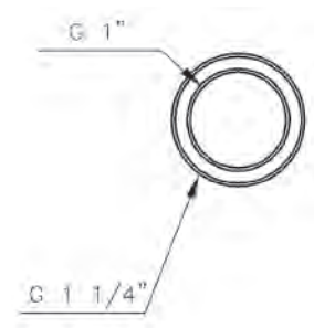
Ref.: 9908 0046 Adaptador sifon 1 1/4" - 1" Siphon adaptor 1 1/4" - 1"
