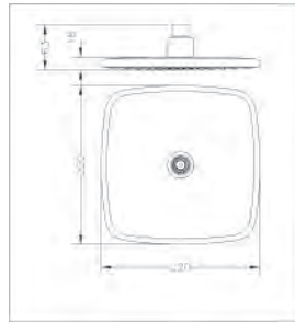
Ref.: R63112 08 Rociador ovalado 22 cm Oval shower head 22 cm Box: 1 | Carton: 24 | Pallet: 192
