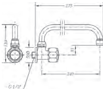
Ref.: 68093 11 45 66 Grifo mural fregadera caño tubo alto 24 cm Wall sink tap with tube spout 24 cm Box: 1 | Carton: 10 | Pallet: 240
