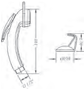
Ref.: 100696 45 Kit ducha sanitaria Sanitary shower kit Box: 1 | Carton: 100 | Pallet: 1800
