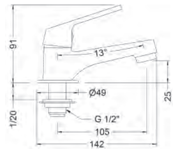
Ref.: 1002 04 Grifo lavabo 1 agua cartucho 25 One-water wash-basin tap 25 cartridge
