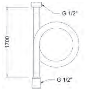
Ref.: 100135 60 00 Flexo H 1/2" - H 1/2" 1,70 m inoxidable F 1/2" - F 1/2" Stainless steel flexible hose 1.70 m
