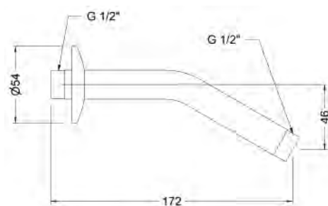
Ref.: 1699 45 00 Brazo pared redondo 12 cm Round wall arm 12 cm
