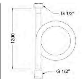
Ref.: 100141 45 Flexo H 1/2" - H 1/2" 1,20 m inoxidable F 1/2" - F 1/2" Stainless steel flexible hose 1.20 m
