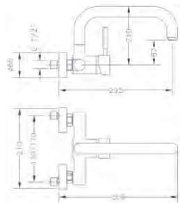
Ref.: 65192 18 45 66 Monomando de fregadera mural 15 cm Wall single lever sink mixer 15 cm
