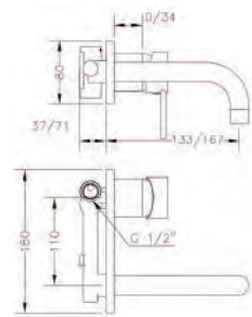
Ref.: 65131 29 45 66 Monomando de lavabo empotrado caño 16 cm Built-in wash-basin mixer 16 cm spout
