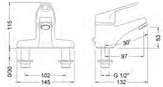
Ref.: 60188 22 45 66 Monomando de lavabo centerset 4" Single lever wash-basin mixer 4" centerset
