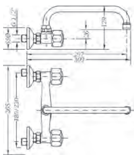
Ref.: 68104 11 45 66 Grupo mural fregadera 20 cm caño tubo alto 24 cm 20 cm wall sink mixer with high tube, 24 cm spout Box: 1 | Carton: 10 | Pallet: 240
