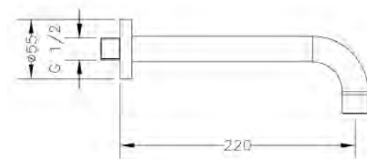
Ref.: 68912 45 Caño mural tubo recto 22 cm Wall mounted pipe spout 22 cm
