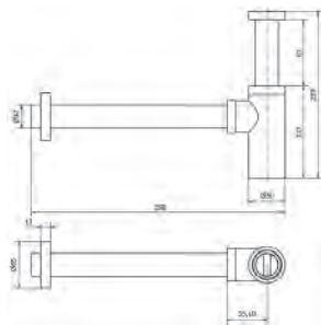
Ref.: 1622 07 Sifon botella para lavabo y bidé 1 1/4" 1 1/4" bidet and wash-basin siphon
