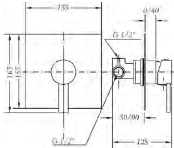
Ref.: 65115 29 45 66 Monomando de ducha empotrado Built-in single lever shower mixer
