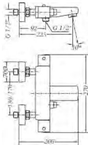
Ref.: 67100 26 45 67 Termostática de baño sin kit Thermostatic bath mixer without kit
