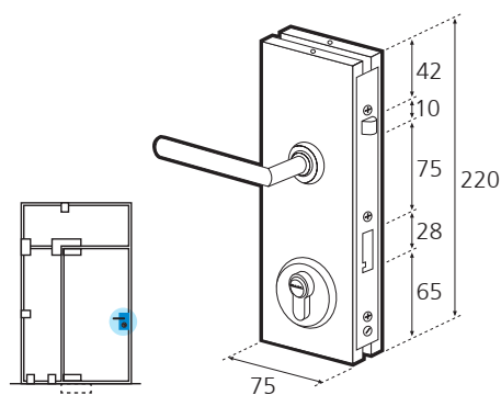
Cerradura DUO-GLASS DUO-GLASS lock DUO-GLASS serrure
