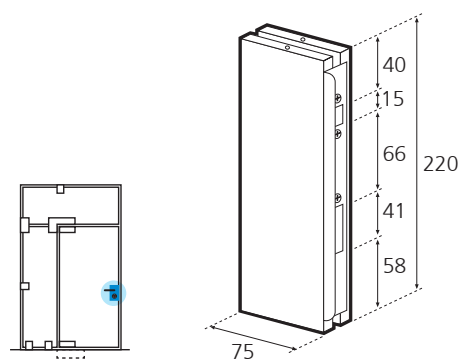
Cerradero a vidrio DUO-GLASS DUO-GLASS lock keeper DUO-GLASS gache pour verre
