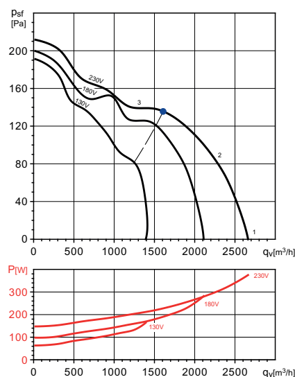
CQ /6 9/9 200W
