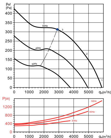
CQ /6 12/12 1100W
