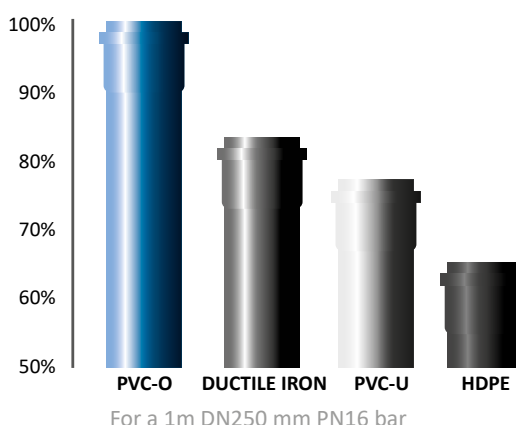
Hydraulic capacity
