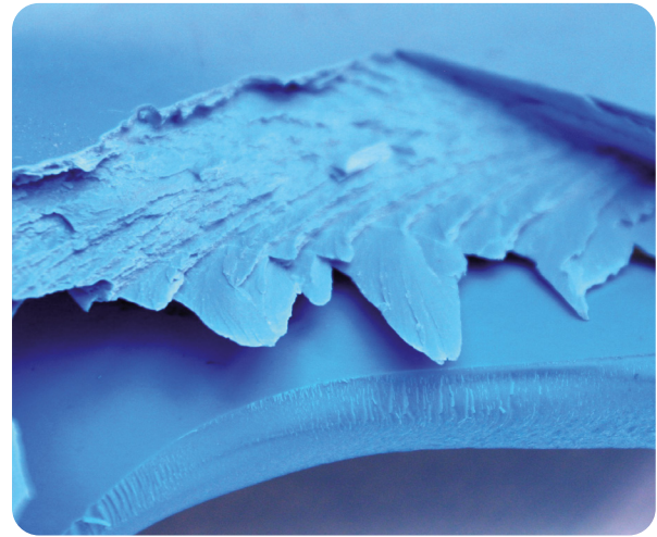
When PVC with its amorphous structure (lower section) is subjected to the orientation process, a laminate structure is obtained (upper section).
