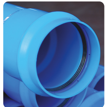
Locked-in ring seals ensure a perfect water-tight fit.
