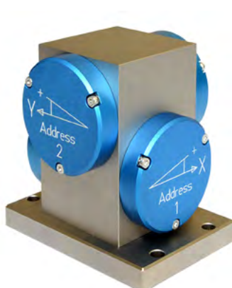
ZEROTRONIC sensor in 2D application
