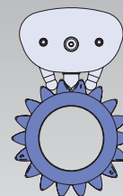
Pitchline clamping with clamping pin
