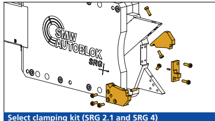
Select clamping kit (SRG 2.1 and SRG 4)
