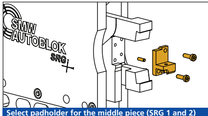
Select padholder for the middle piece (SRG 1 and 2)
