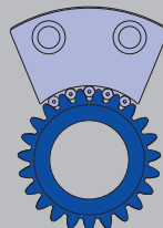
Pitchline clamping with roller cage
