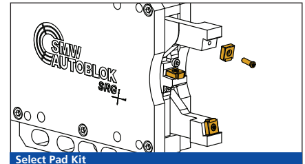
Select Pad Kit
