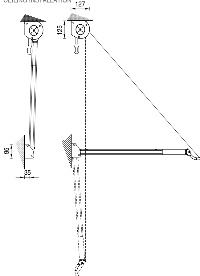
MONTAJE A TECHO CEILING INSTALLATION
