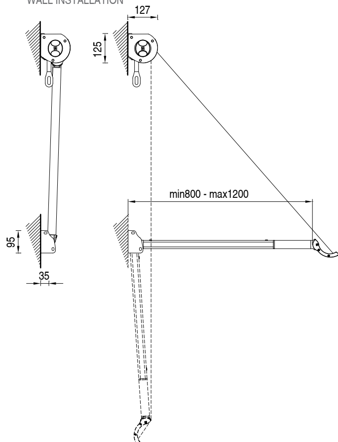
MONTAJE A PARED WALL INSTALLATION
