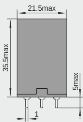
Circuito impreso, 3C
