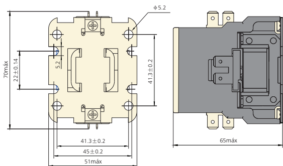
NCK3-25/1P~40/1P
