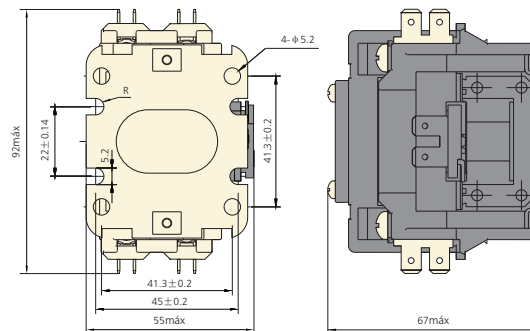
NCK3-25/1~40/1
