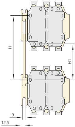
b. NC2-265Nc~630Nc
