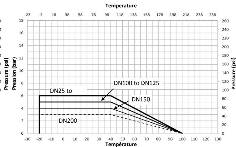
PVDF
