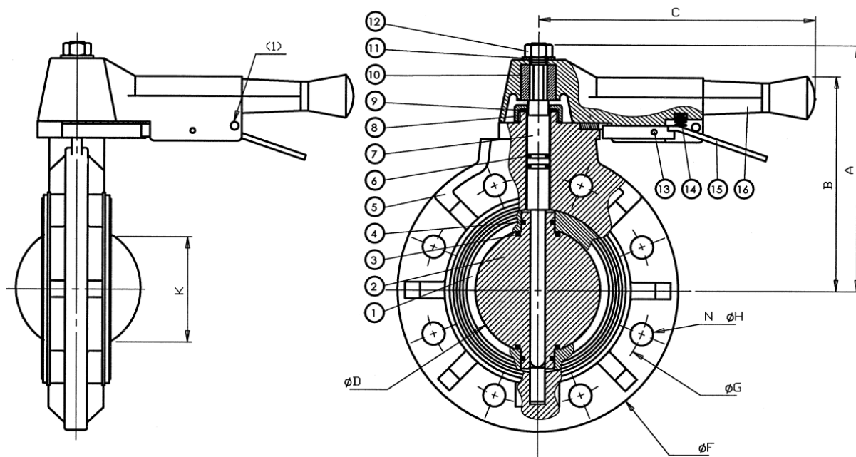
Diagram representing a DN150
