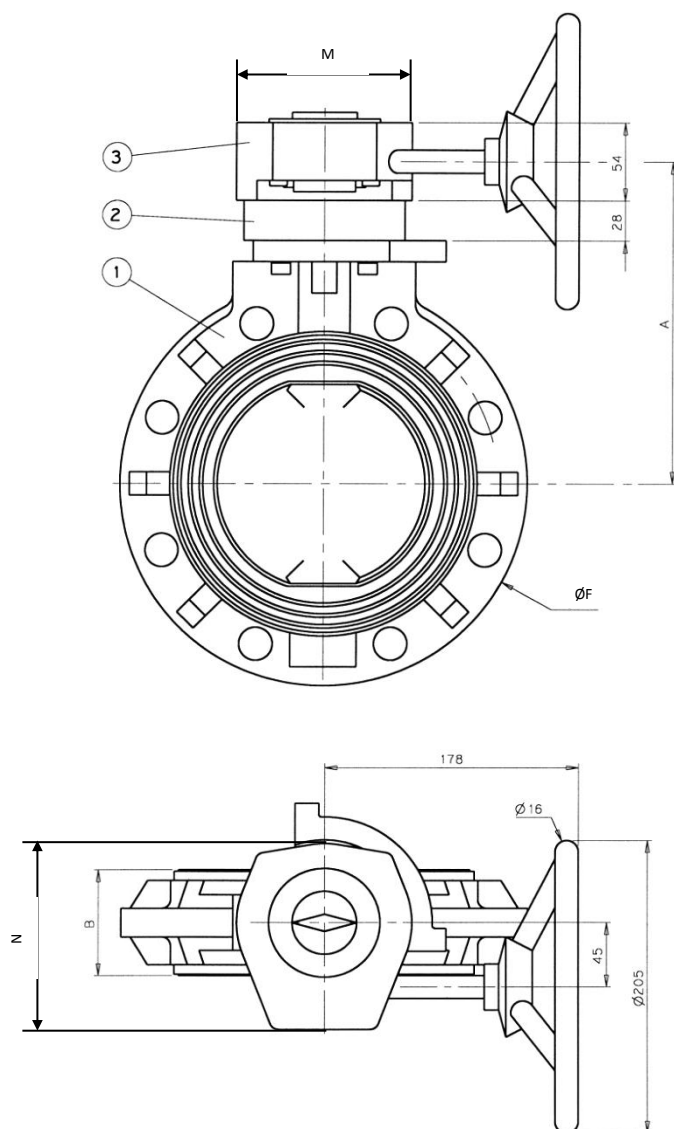
Diagram representing assembly on a DN200
