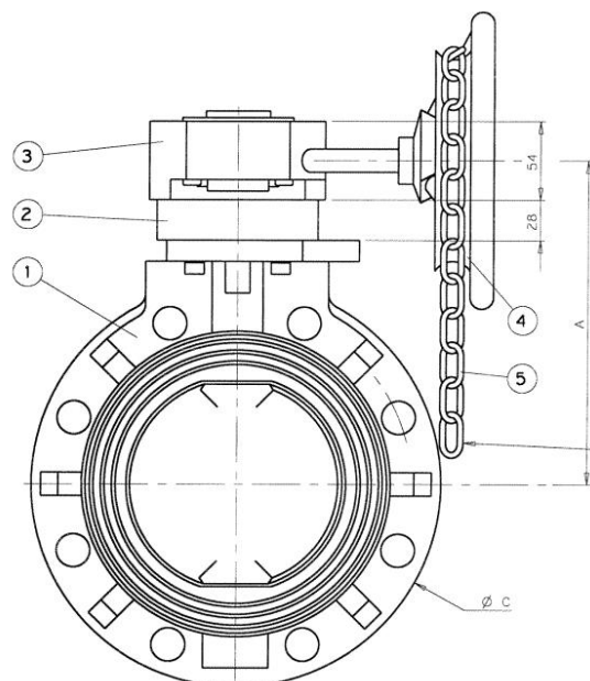
Chain Operation
