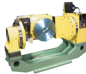
5AX-500MA-RJ10-900/100
