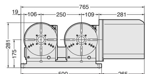
CNC202-2W
