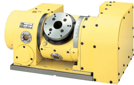
5AX-130FA
