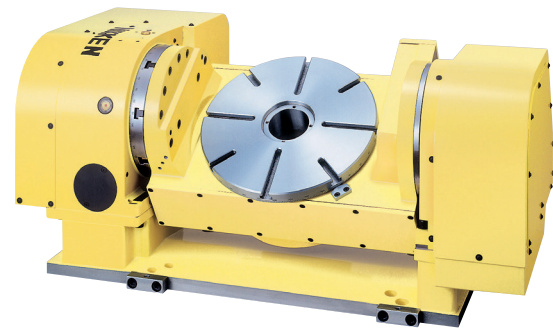
5AX-350
