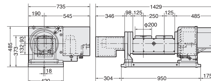
5AX-2MT-200-250
