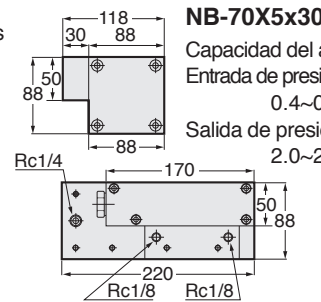
NB-70X5X30
