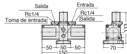
NBH-100X
