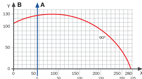
Diagramma di taglio Cutting diagram/Diagramme de coupe Diagrama de corte/Schnittt diagram
