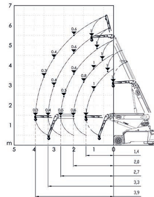
MANUAL JIB
