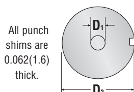
114 PUNCH SHIM PACKAGE
