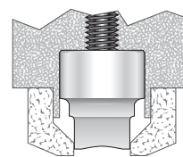
Urethane Stripper Profile for Square Punches - Four Walls Reinforced
