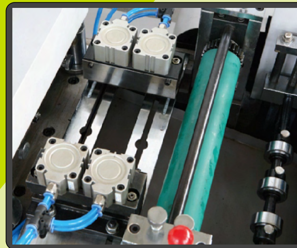
Pistones ajustables
