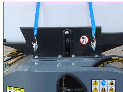
▲ Sistema flotante del acoplamiento Floating system for the adaptation
