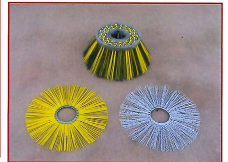
▲ Discos cepillo central y cepillo lateral Discs central brush and side sweeper
