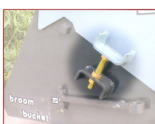
▲ Sistema regulación cepillo central Adjusting system for the central brush
