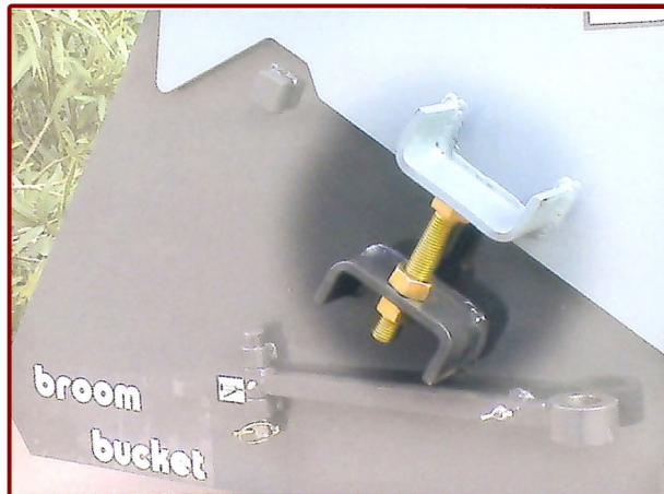
▲ Sistema regulación cepillo central Adjusting system for the central brush
