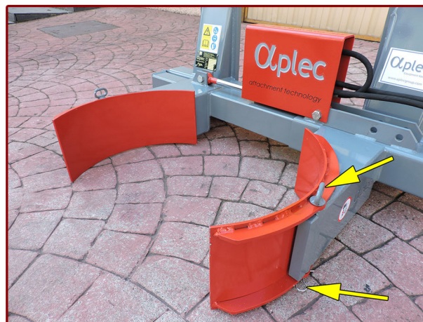
▲ Mordazas desmontables / Removable jaws
