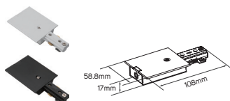
Conector/Connector
