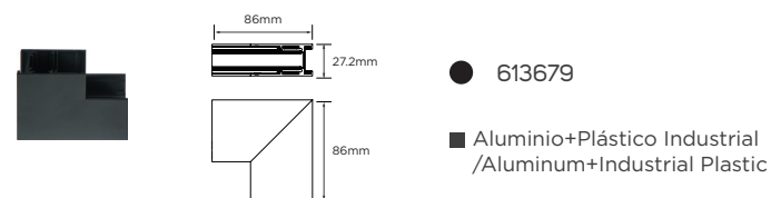
Esquina interior montada en superficie//Surface Mounted Inside Corner
