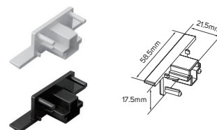
Tapa final/End Cap
