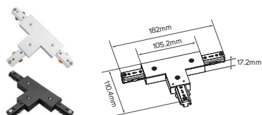
Conector/Connector
