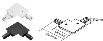
Conector/Connector
