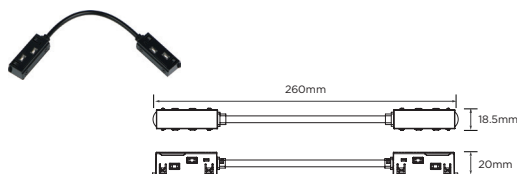
Módulo conductor de esquina flexible IP20/Flexible Corner Conductive Module
