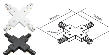
Conector/Connector
