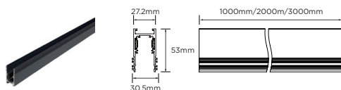
Carril magnético empotrado/Recessed Magnetic Track Rail
