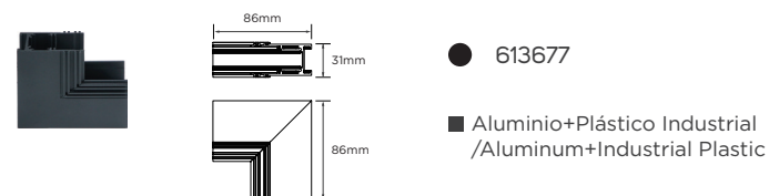
Esquina interior empotrada/Recessed Inside Corner
