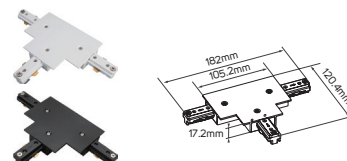
Conector/Connector
