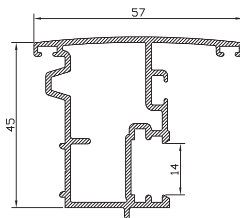
INVERSOR CURVO 22385
