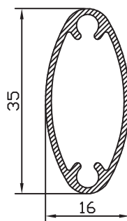
VERTICAL OVOIDE 55008
