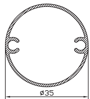
VERTICAL REDONDO 55009
