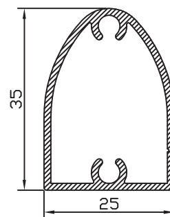
VERTICAL SEMI-OVOIDE 55016
