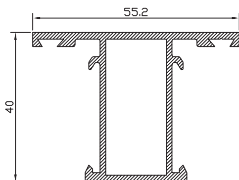
PILASTRA 40x20 1.8 32584
