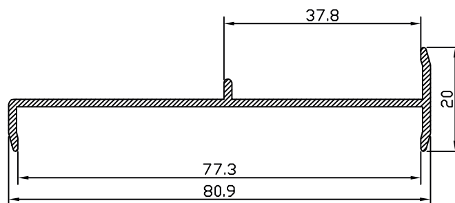
UNION CORREDERA ABATIBLE 24005
