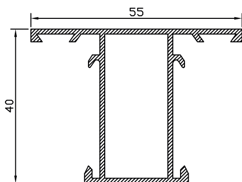
PILASTRA 55 32580
