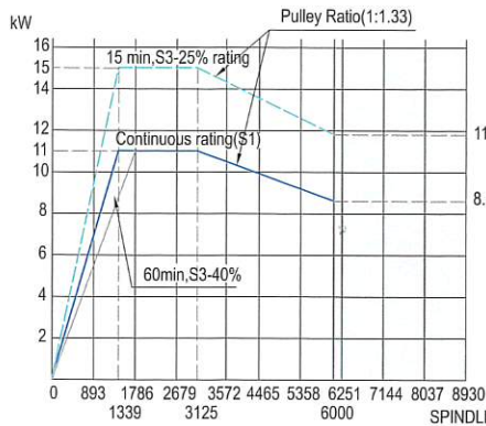
Horsepower Chart
