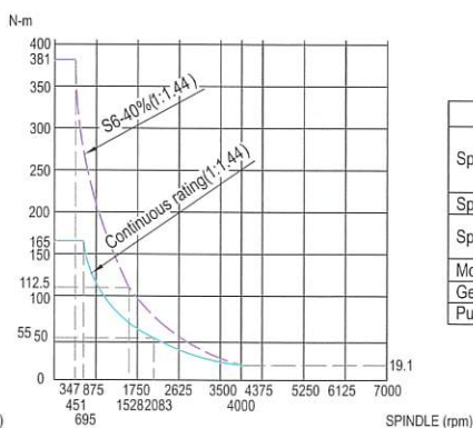
Torque Chart
