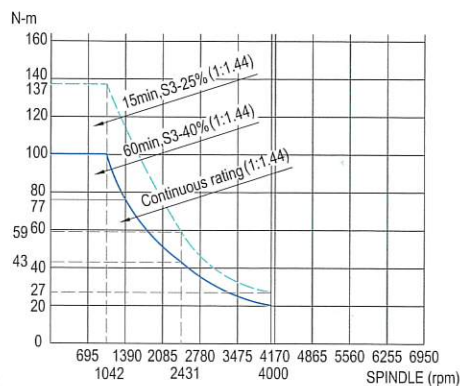
Torque Chart
