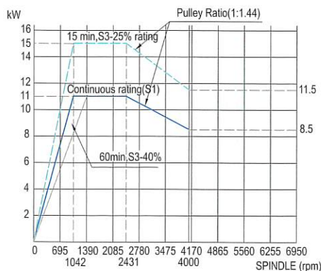
Horsepower Chart
