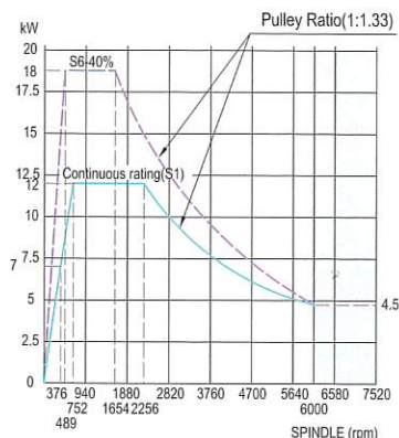
Horsepower Chart
