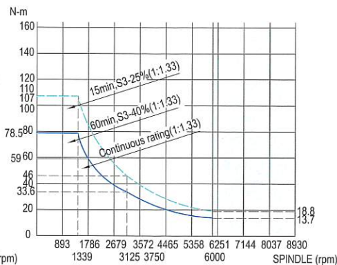
Torque Chart
