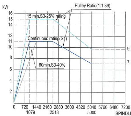
Horsepower Chart
