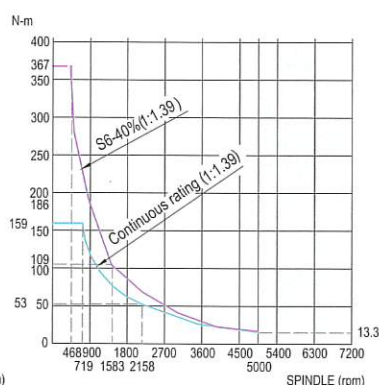
Torque Chart
