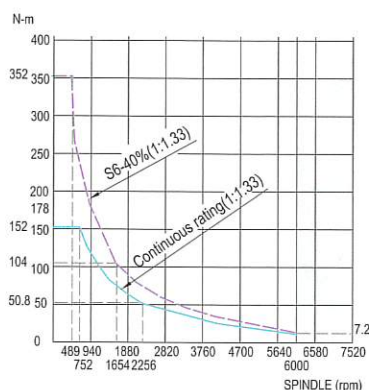
Torque Chart
