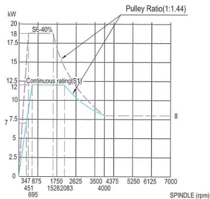
Horsepower Chart
