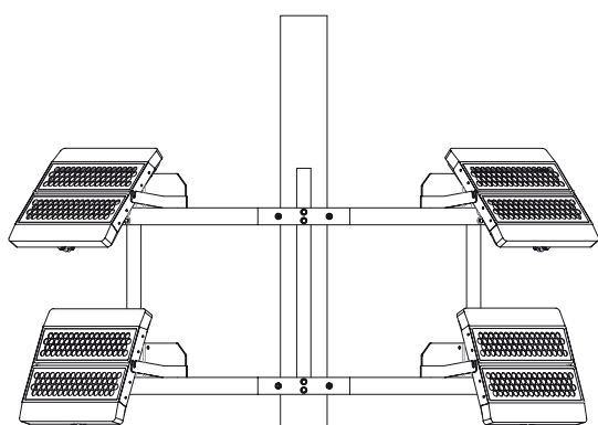
Custom made brackets for 4 Square Grazers® 66x2
