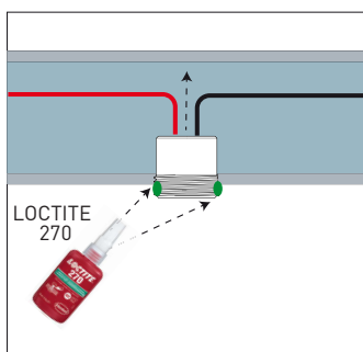
Loctite 270 sealer threads (ref. M020081) Loctite 270 sellador roscas (ref. M020081)
