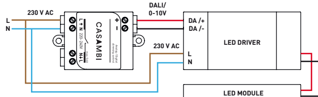
Wiring diagram, directly powered DALI or 0-10V drivers Suitable for drivers that can be switched off via control interface
