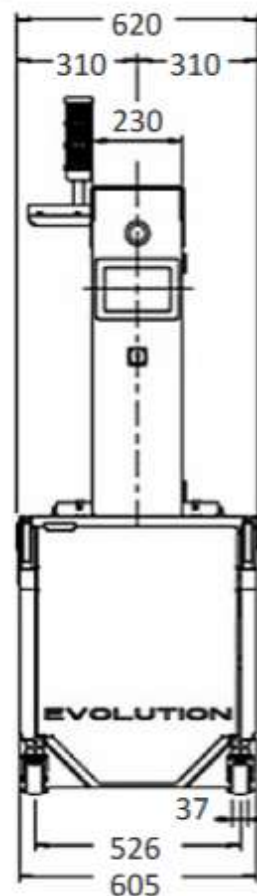
Plano TR-6 PRO / 600 mm x 600 mm
