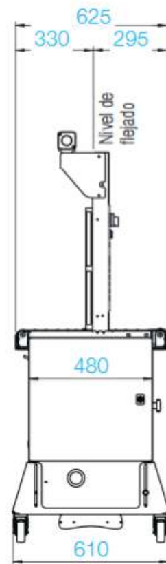
SoniXs MP-6 R (600 x 600 mm)
