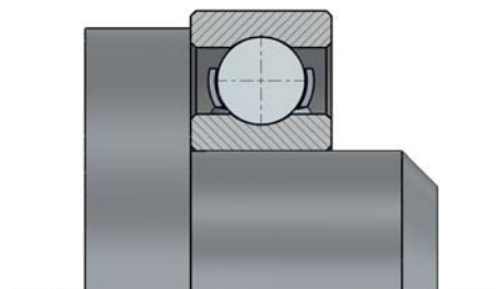
Wrong, Shaft shoulder greater than d_{a\max}
