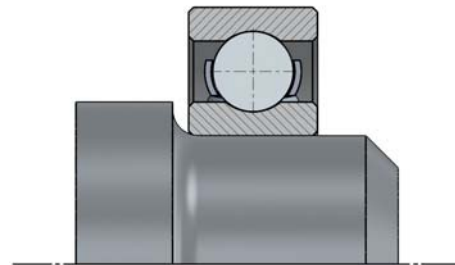
Wrong, Shaft radius greater r_{s\min}
