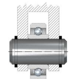
Bearings with extended inner ring
