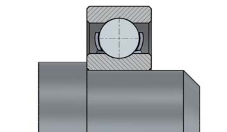
Wrong, Shaft shoulder smaller than d_{a\min}
