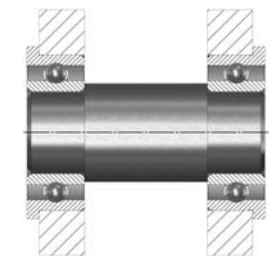
Assembly in narrow housings
