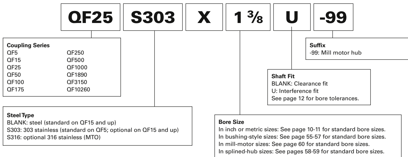
Fig. 11. Hubs.
