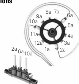
Fig 28. Suggested pump element positions
