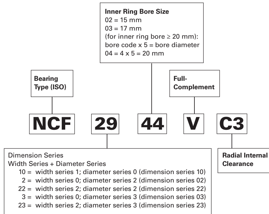
Fig. 19. Full-complement (NCF) cylindrical roller bearing nomenclature.
