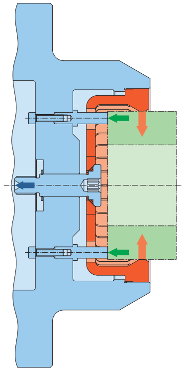
Basket Element Clamping Chuck
