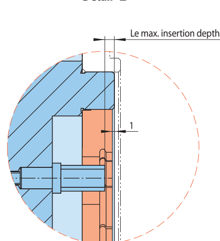
Detail "Z"
