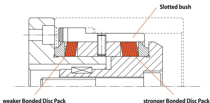
weaker Bonded Disc Pack stronger Bonded Disc Pack
