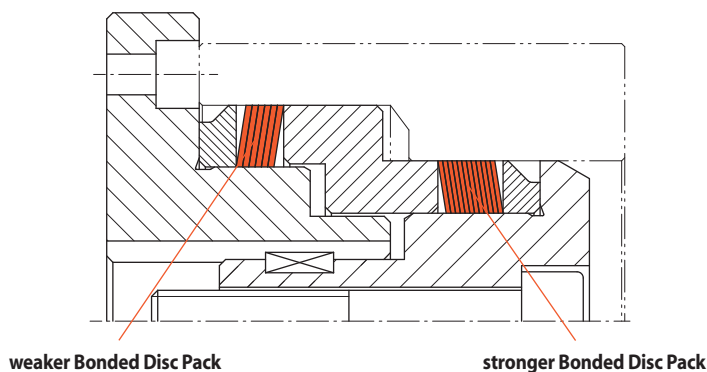
weaker Bonded Disc Pack stronger Bonded Disc Pack
