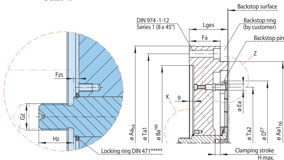
Detail "X"
