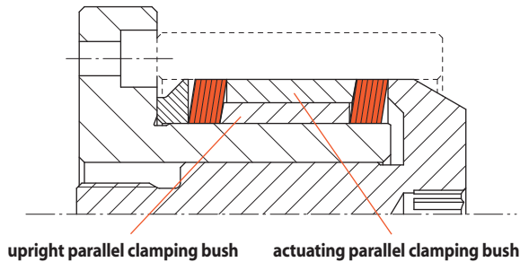
upright parallel clamping bush actuating parallel clamping bush
