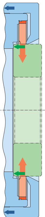
Disc Element Clamping Chuck
