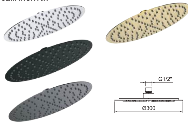
Rociador ducha Slim Inox Air Ø300mm. Slim Inox Air head shower Ø300mm.
