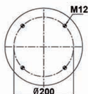
INFERIOR / BOTTOM VIEW
