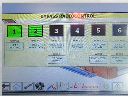
Control panel with smart user interface and remote assistance device for both the shredder and the Scania motor
