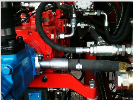
Hydraulic transmission with variable speed
