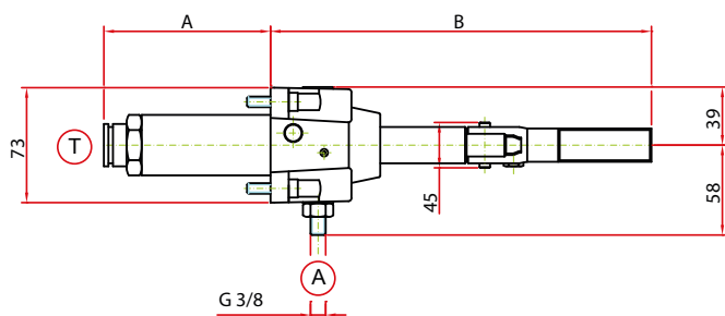
SOPORTE PARA DEPOSITO REMOTO SUPPORT FOR REMOTE TANK
