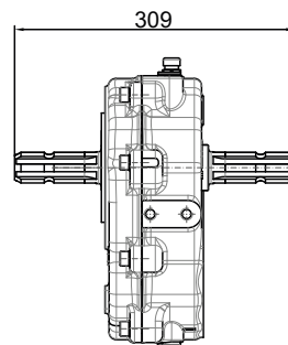
Eje Macho / Macho Male Shaft / Male
