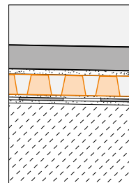
Schlüter®-DITRA-DRAIN 8
