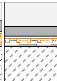
Schlüter®-DITRA-DRAIN 4
