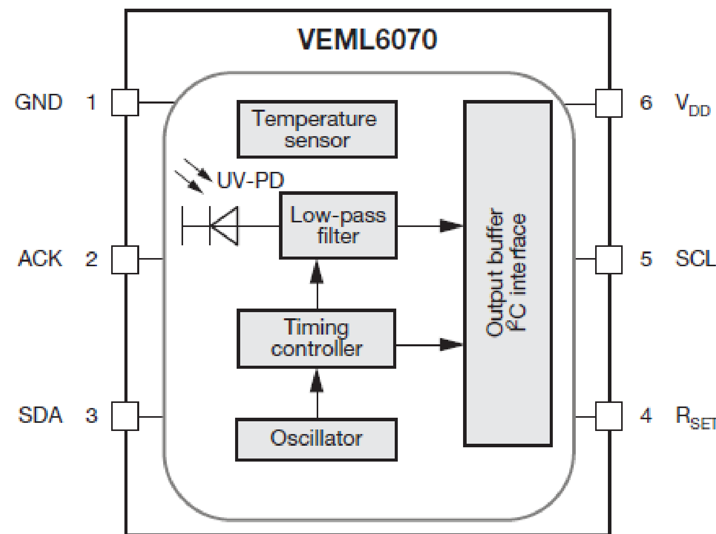
Fig. 1 - Block Diagram of the VEML6070
