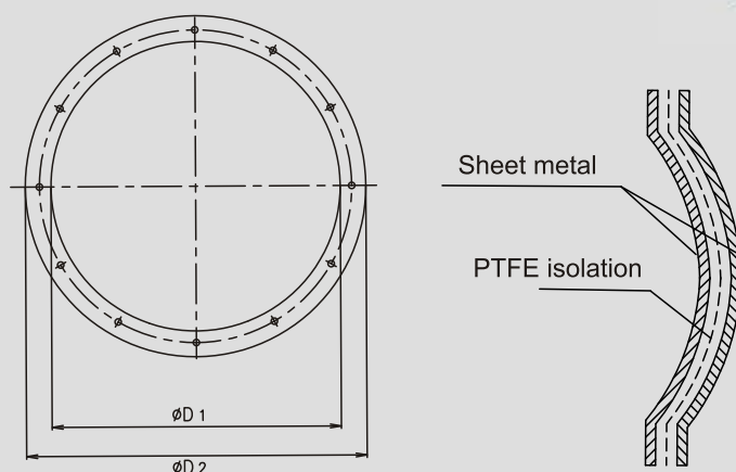
Technical data - round VMP panels
