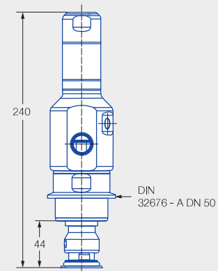
Tri-Clamp connection 5P9
