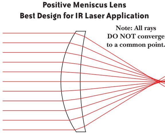
Figure 3 Spherical aberration
