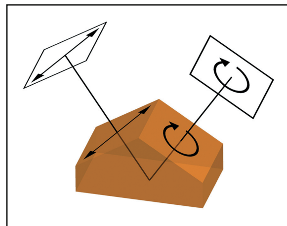
This quarter-wave prism converts linear into circular polarization, and turns the beam path.
