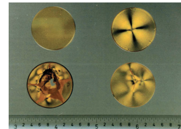
Starting clockwise at the top left: The progression of a thermally stressed lens.
