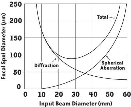
Figure 4 Spot size due to aberration and diffraction
