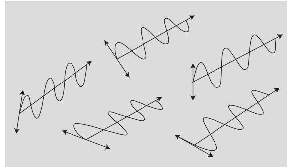
Figure 2 Unpolarized light
