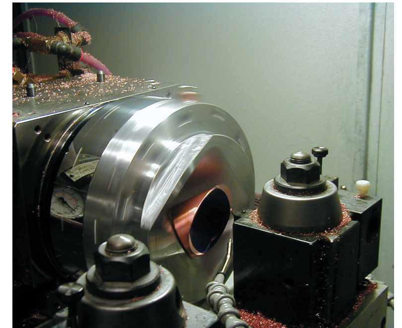
A long-working-distance parabolic mirror is cut with II-VI Infrared's slow-tool servo.
