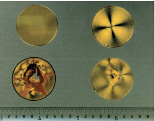
Starting clockwise at the top left: The progression of a thermally stressed lens.
